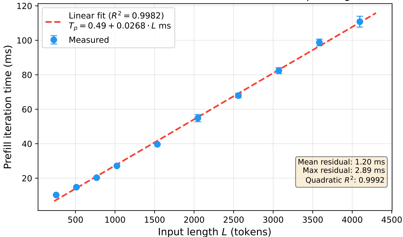
Qwen/Qwen3-8B (H200) — Prefill time vs. input length
