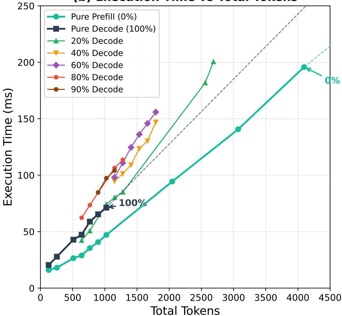
(b) Execution Time vs Total Tokens
