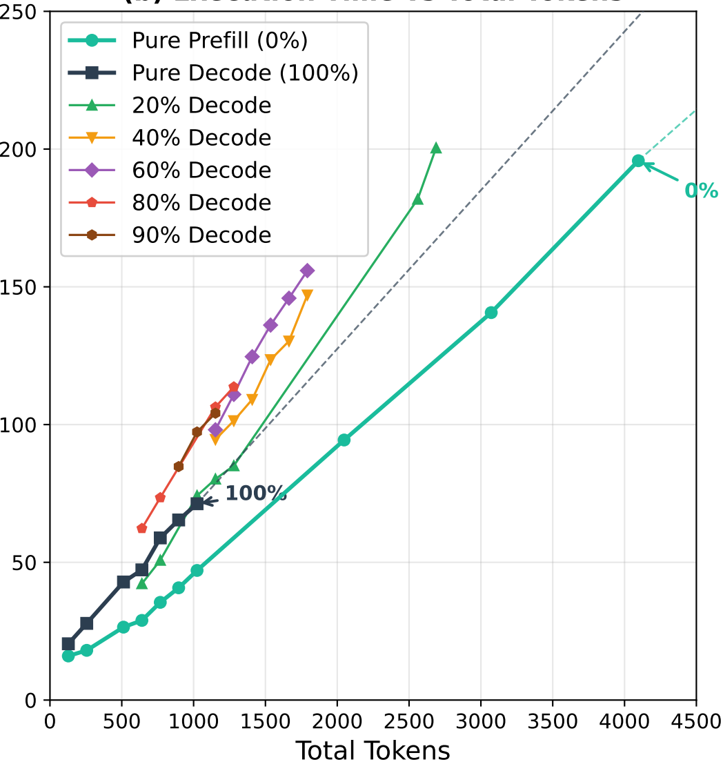
(b) Execution Time vs Total Tokens
