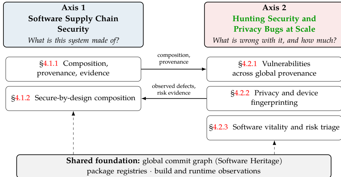
Figure 1: The CUNCUN research programme: two coupled axes over one shared foundation. Axis 1 establishes what a system is composed of and how it should be composed; Axis 2 finds and prioritises what is wrong with it. Provenance flows left to right; evidence about observed defects flows right to left.
