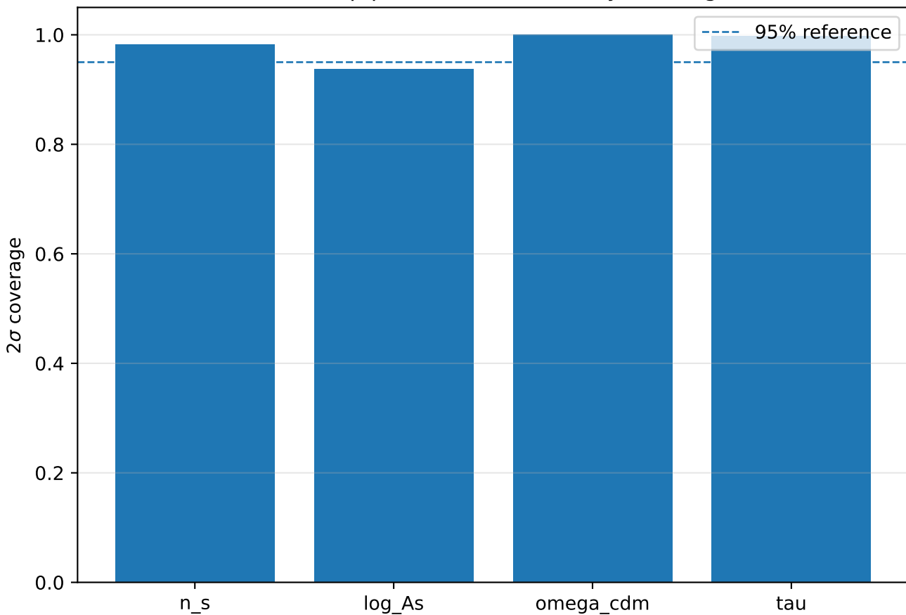
Bootstrap predictive-uncertainty coverage
