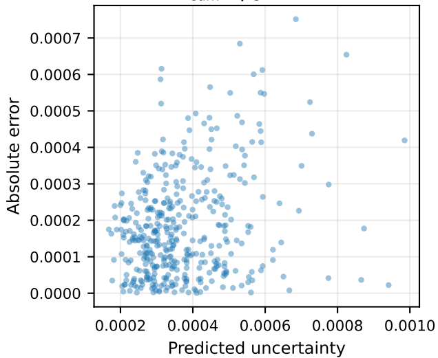
\omega_{\text{cdm}} ( \rho_s = 0.18 )
