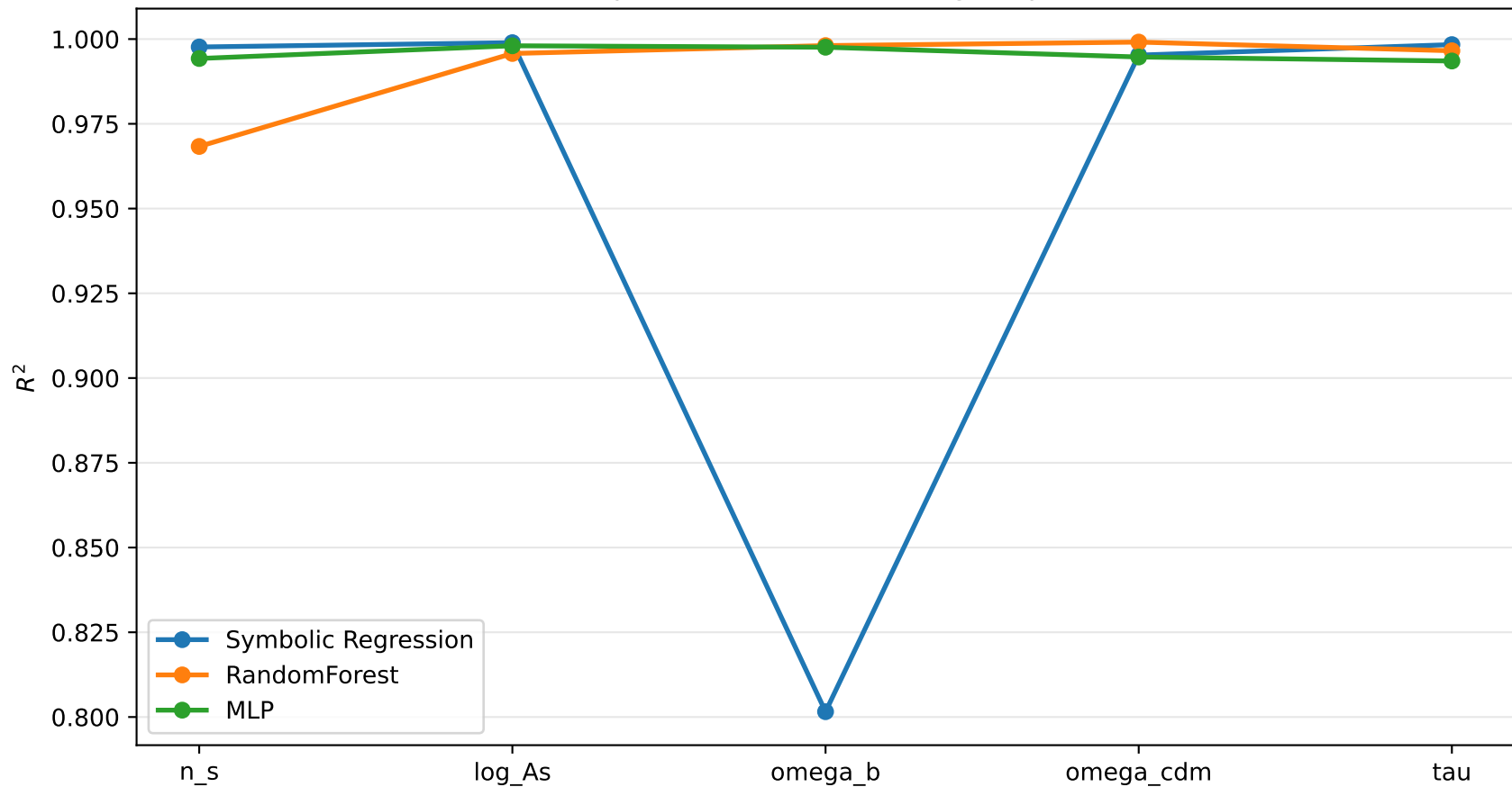
Model comparison across cosmological parameters
