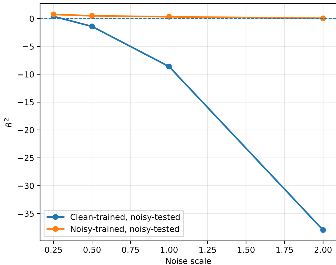
Noise robustness: n_s
