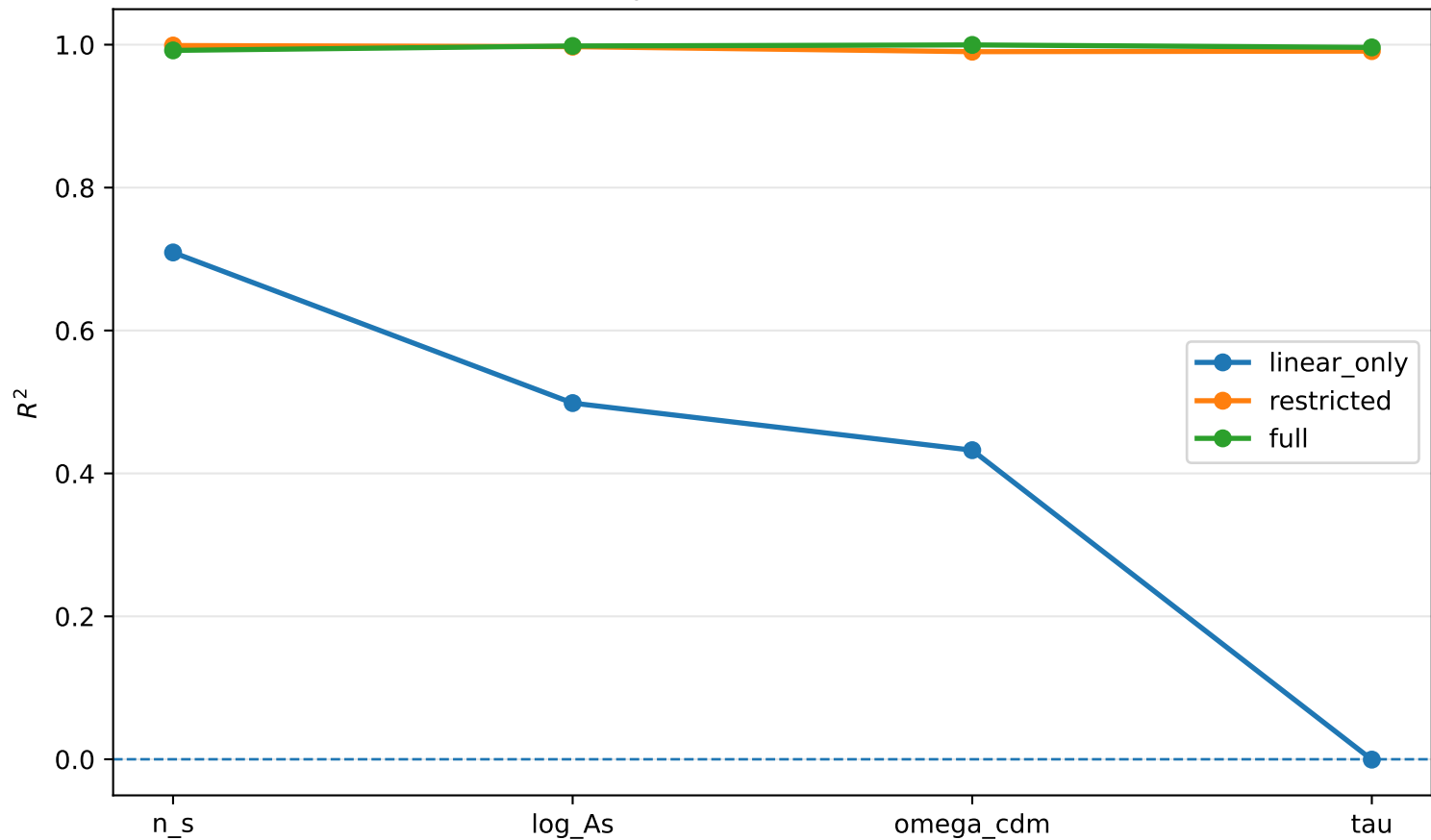
Operator-set ablation
