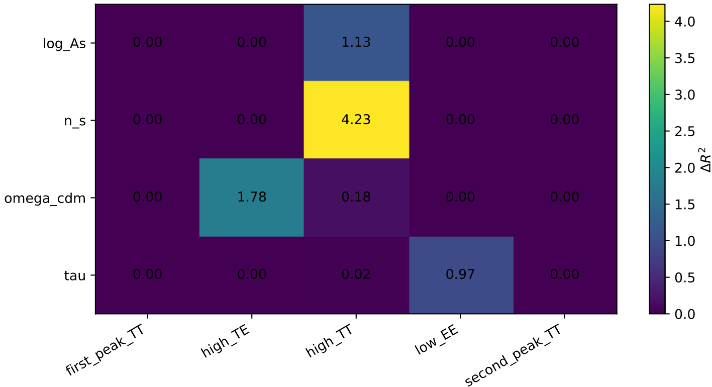
Perturbation-based interpretability test
