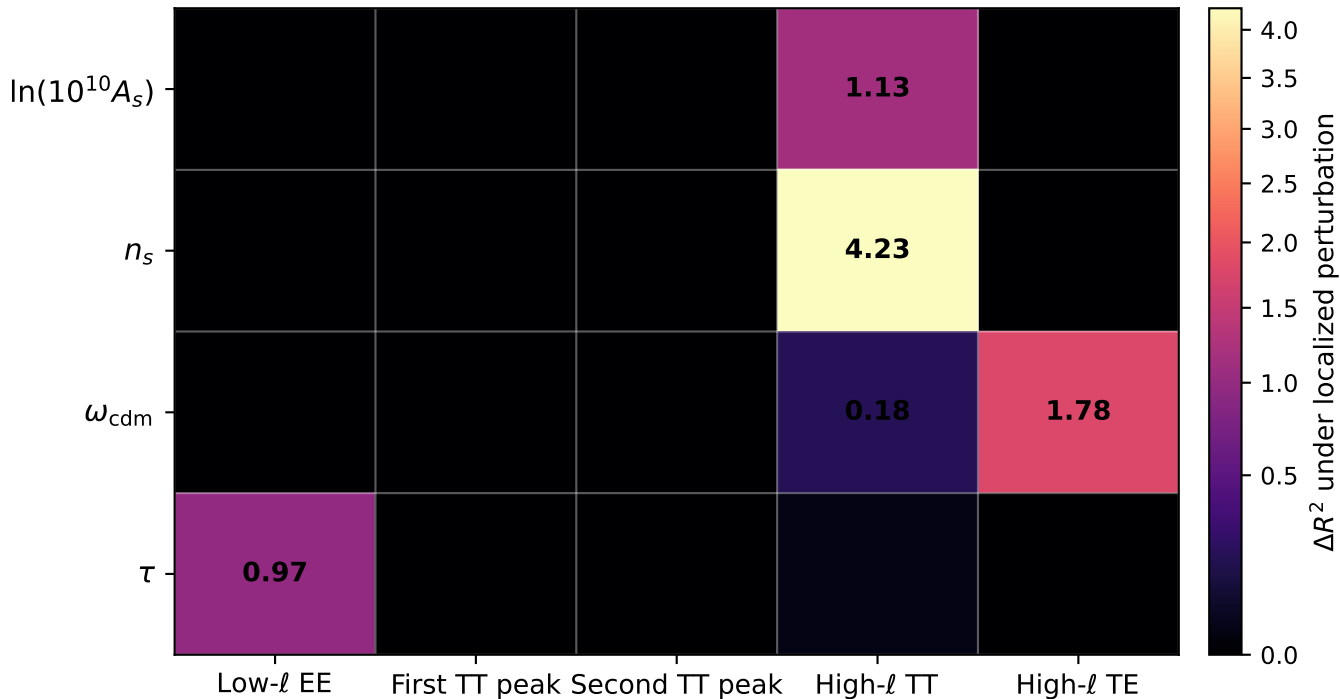
Region-wise sensitivity of cosmological parameter inference
