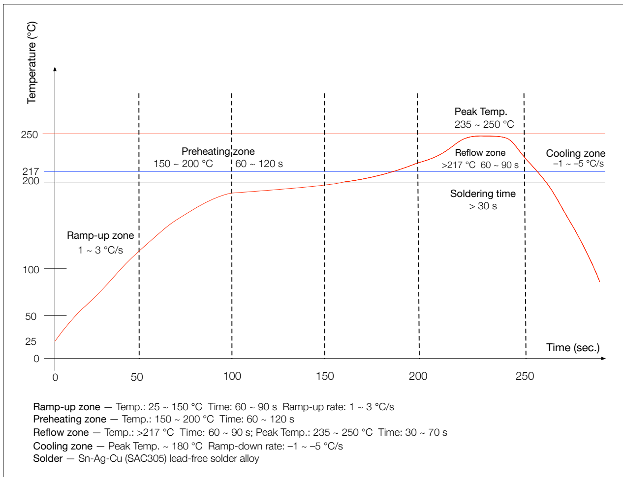
Figure 16: Reflow Profile
