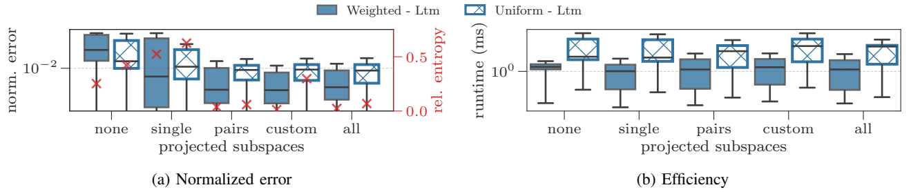
Fig. 14: Effect of the selection of projected numerical subspaces on the accuracy and runtime of PACHA SKETCHES.
