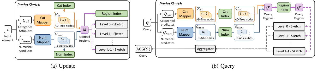
Fig. 4: PACHA SKETCHES illustration for answering for (a) Update: each tuple is mapped based on the categorical (orange) and numerical (blue) regions, updating the indexing structures and the base sketches at every level. (b) Query: categorical predicates map to AD-tree nodes, numerical predicates map to \mathbb{B} -adic cubes, and the union of these regions is queried in the base sketches.
