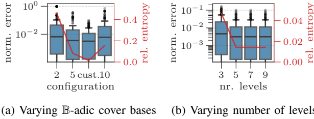
Fig. 15: Accuracy with different parameters.
