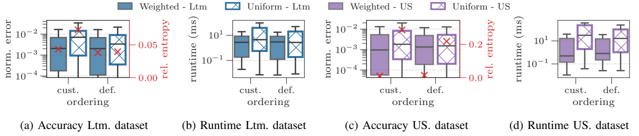
Fig. 12: Effect of attribute ordering in the AD-tree on the accuracy and runtime of PACHA SKETCHES.
