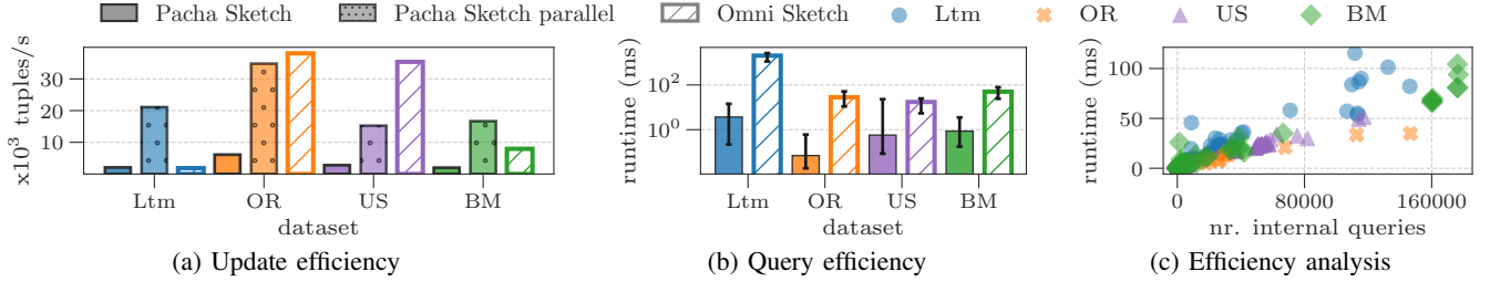
Fig. 8: Update and query efficiency across different datasets.
