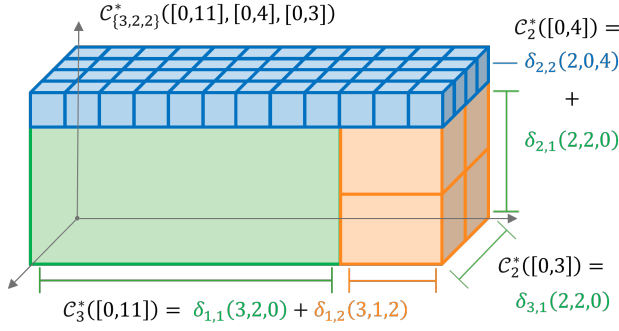
Fig. 2: \mathbb{B} -adic space cover ( \mathbb{B} = \{3, 2, 2\} )
