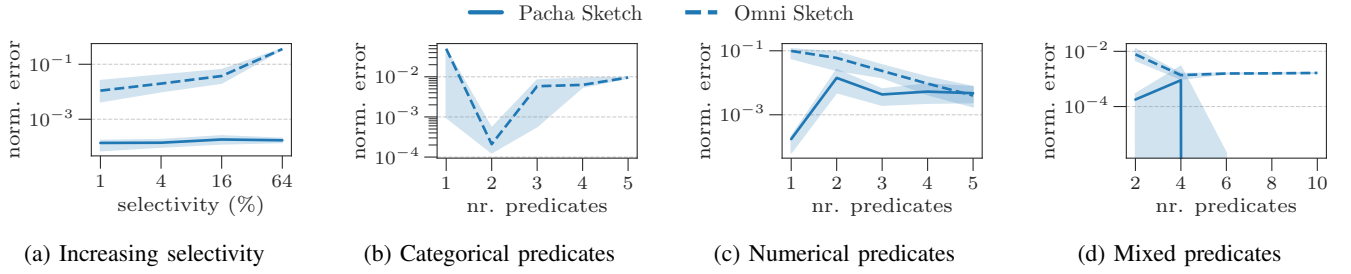
Fig. 7: Accuracy against the state of the art across query workloads.
