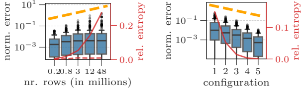
(a) Increasing number of rows. (b) Accuracy guarantees.
