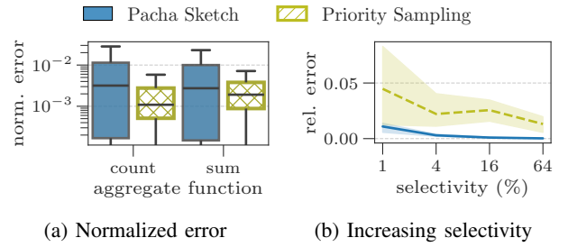
Fig. 9: Accuracy of PACHA SKETCHES (PS) compared to Priority Sampling (S) for different aggr. and selectivities.
