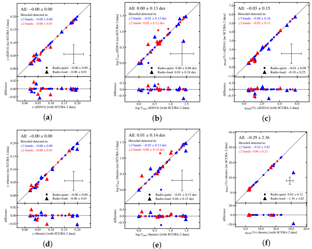
Figure A2. Comparison of the dust-related parameters derived with and without the SCUBA-2 data: (a) \gamma from the Dale2014 template; (b) \log U_{\min} from the Dale2014 template; (c) q_{\text{PAH}} from the Dale2014 template; (d) \gamma from the THEMIS template; (e) \log U_{\min} from the THEMIS template; and (f) q_{\text{HAC}} from the THEMIS template. The lower subpanel in each panel shows the difference between the two estimates. The symbols and colors are the same as in Figure 4.
