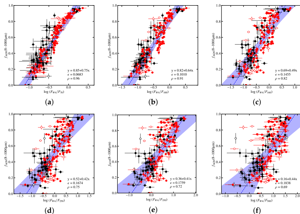
Figure A12. Same as Figure 12 but for WISE W4 and the six Herschel bands: (a) W4/70 \mu\text{m} , (b) W4/100 \mu\text{m} , (c) W4/160 \mu\text{m} , (d) W4/250 \mu\text{m} , (e) W4/350 \mu\text{m} , and (f) W4/500 \mu\text{m} . Red and black symbols denote sources detected in at least three and in no more than two Herschel bands, respectively. Filled and open symbols represent radio-quiet and radio-loud quasars, respectively. The dashed line and blue shaded region show the Bayesian linear regression fit and its uncertainty for the radio-quiet sources detected in at least three Herschel bands. The fitted relation, intrinsic scatter \epsilon , and correlation coefficient \rho are shown in each panel.
