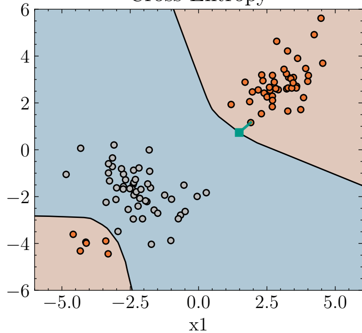
Cross-Entropy
