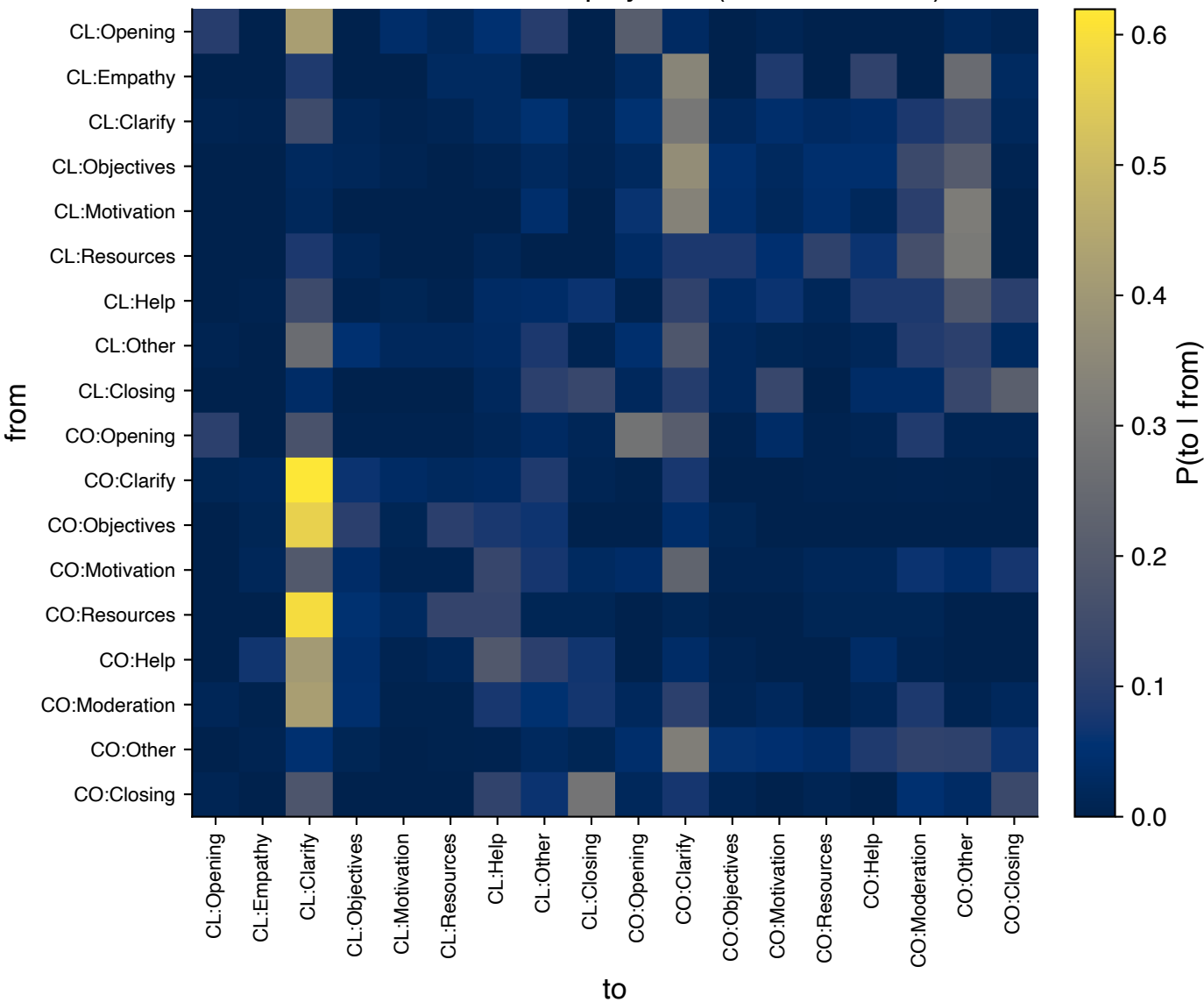
Transitions — HH roleplay chat (row-normalized)
