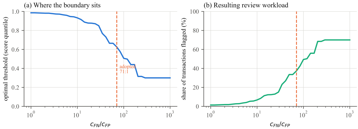
Figure 4. Behaviour of the optimal decision as the cost ratio c_{FN}/c_{FP} is swept over three orders of magnitude. (a) The optimal threshold, expressed as a quantile of the score distribution. (b) The resulting share of traffic flagged for review. The dashed line marks the 71:1 ratio adopted here.
