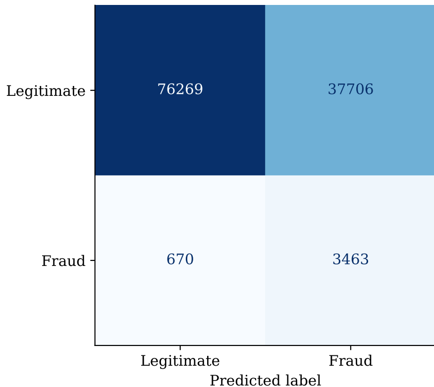
Confusion Matrices at Optimal Cost Threshold \theta^*
