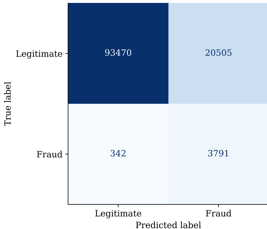
Confusion Matrices at Optimal Cost Threshold \theta^*
