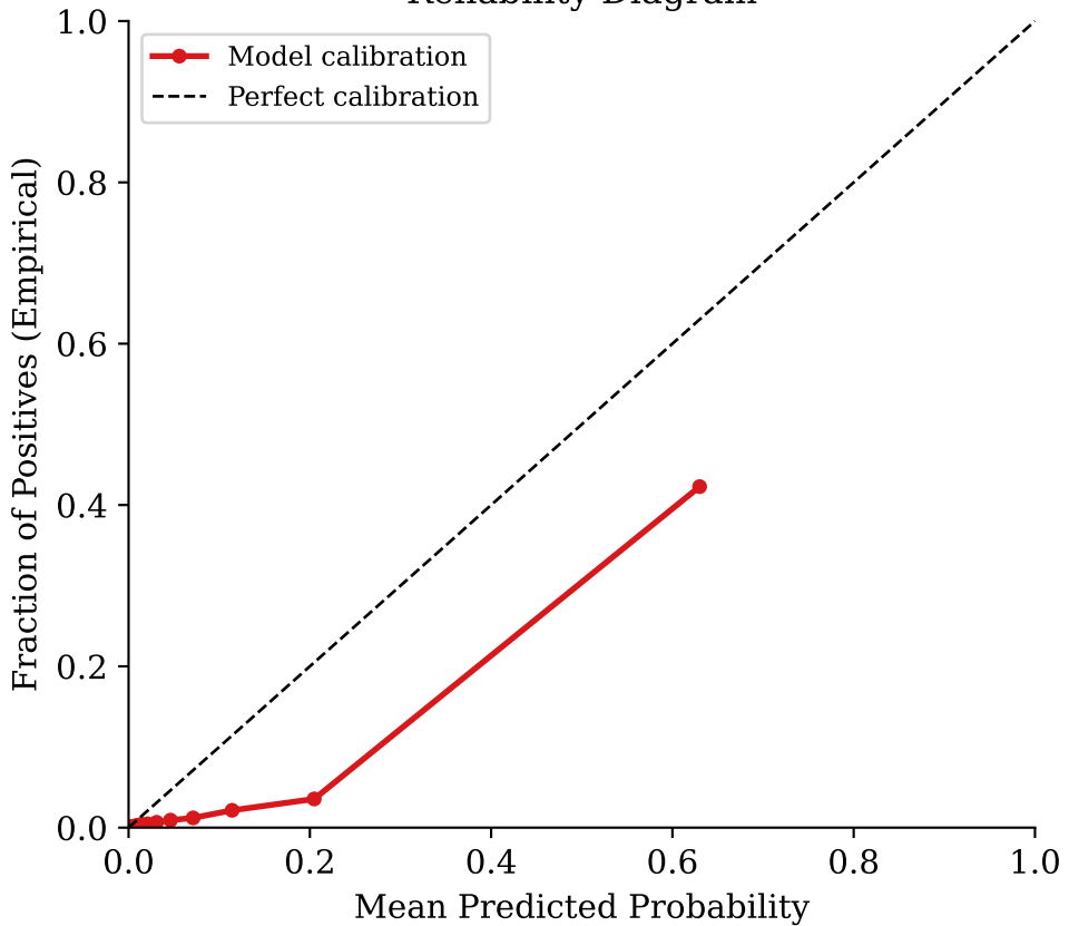
XGBoost Reliability Diagram
