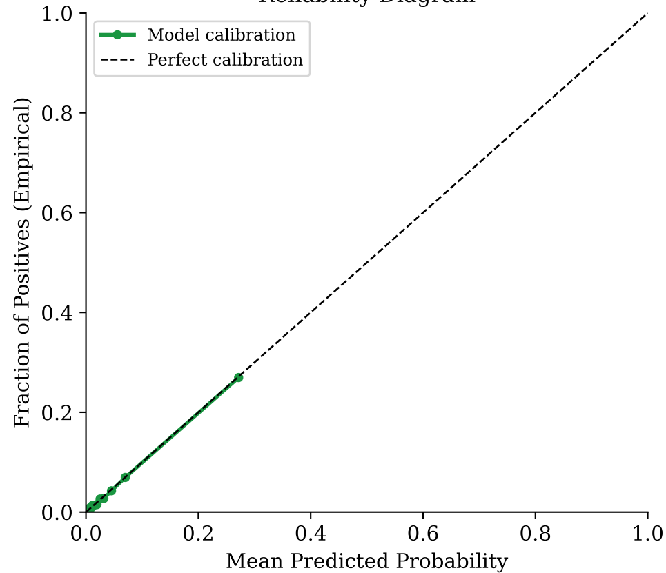
Logistic Regression Reliability Diagram
