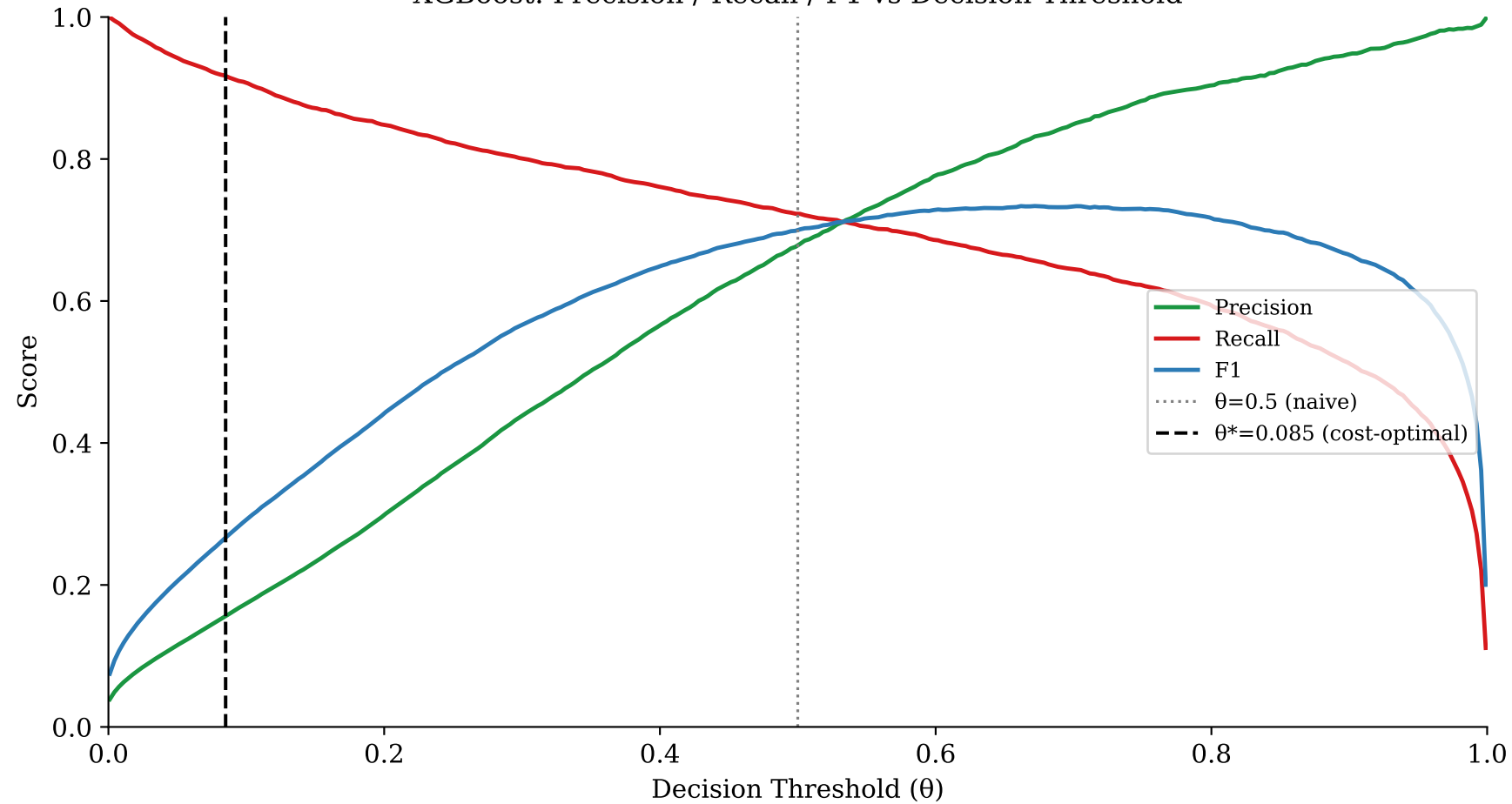
XGBoost: Precision / Recall / F1 vs Decision Threshold
