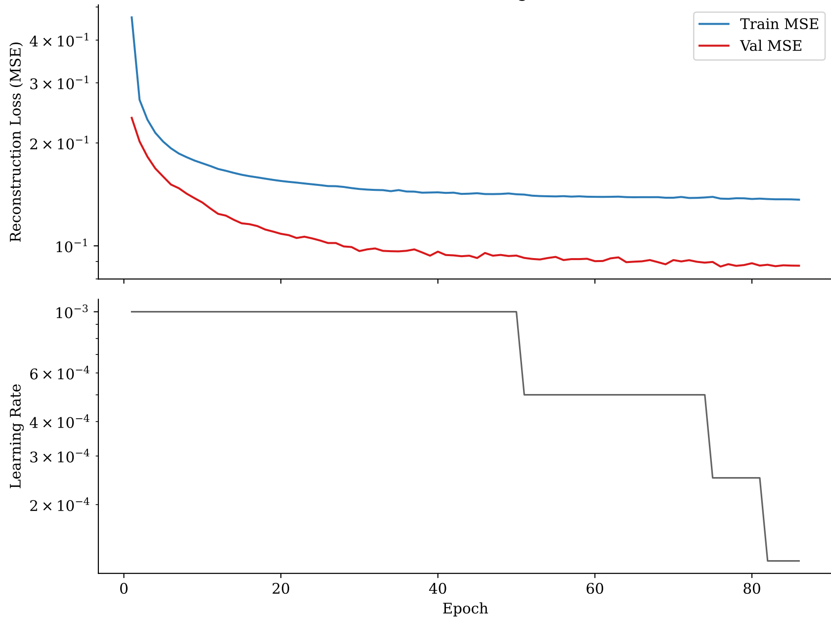
Autoencoder Training Curves
