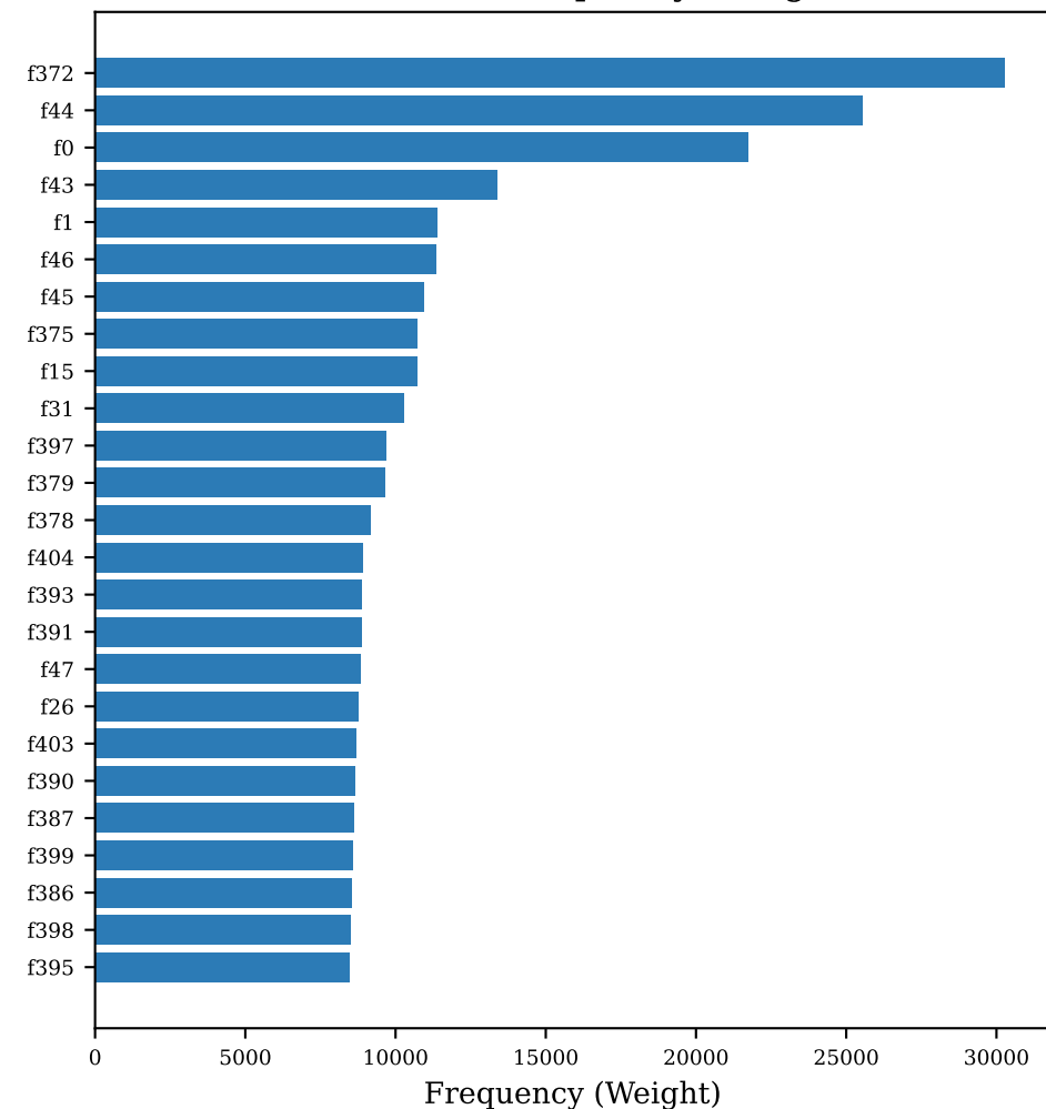
XGBoost — Frequency (Weight)
