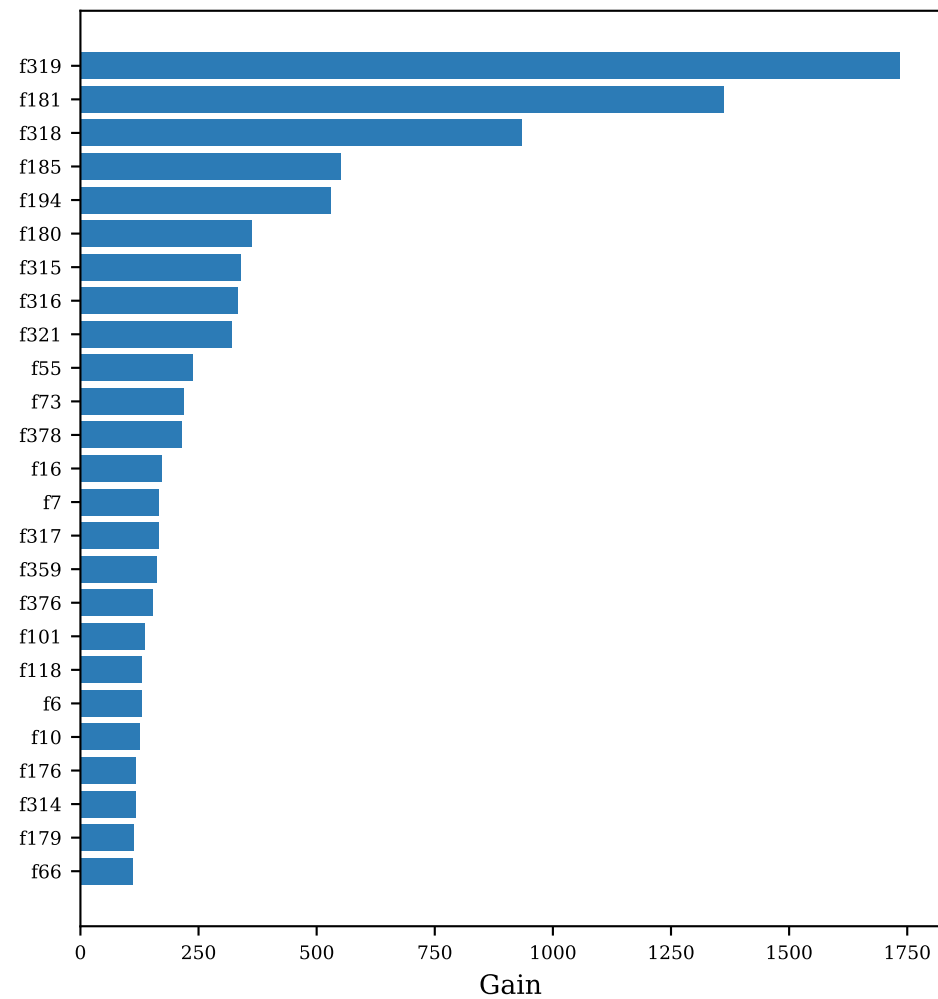
XGBoost — Gain
