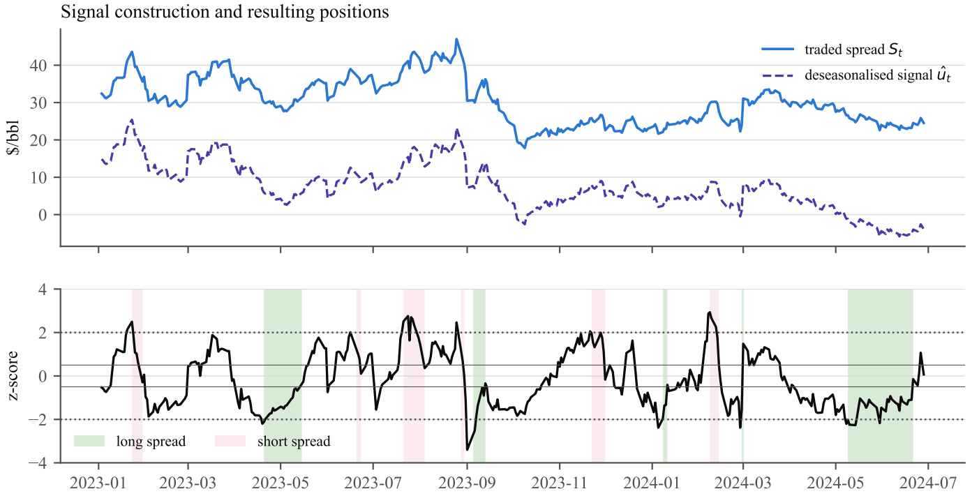
Figure 5. Signal construction and resulting positions over 2023–mid-2024. Upper panel: the traded spread S_t and the deseasonalised signal series \hat{u}_t on which the z-score is computed. Lower panel: the z-score with entry bands at \pm\theta_{\text{en}} and exit bands at \pm\theta_{\text{ex}} ; shaded regions mark executed long and short positions after the one-day execution lag.
