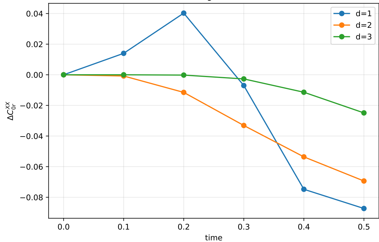
Connected magnetic correlators
