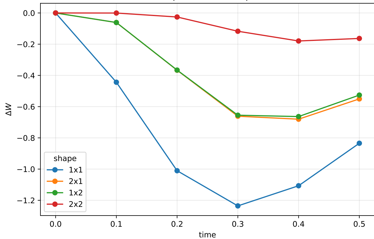
Wilson loops (dual-area X products)
