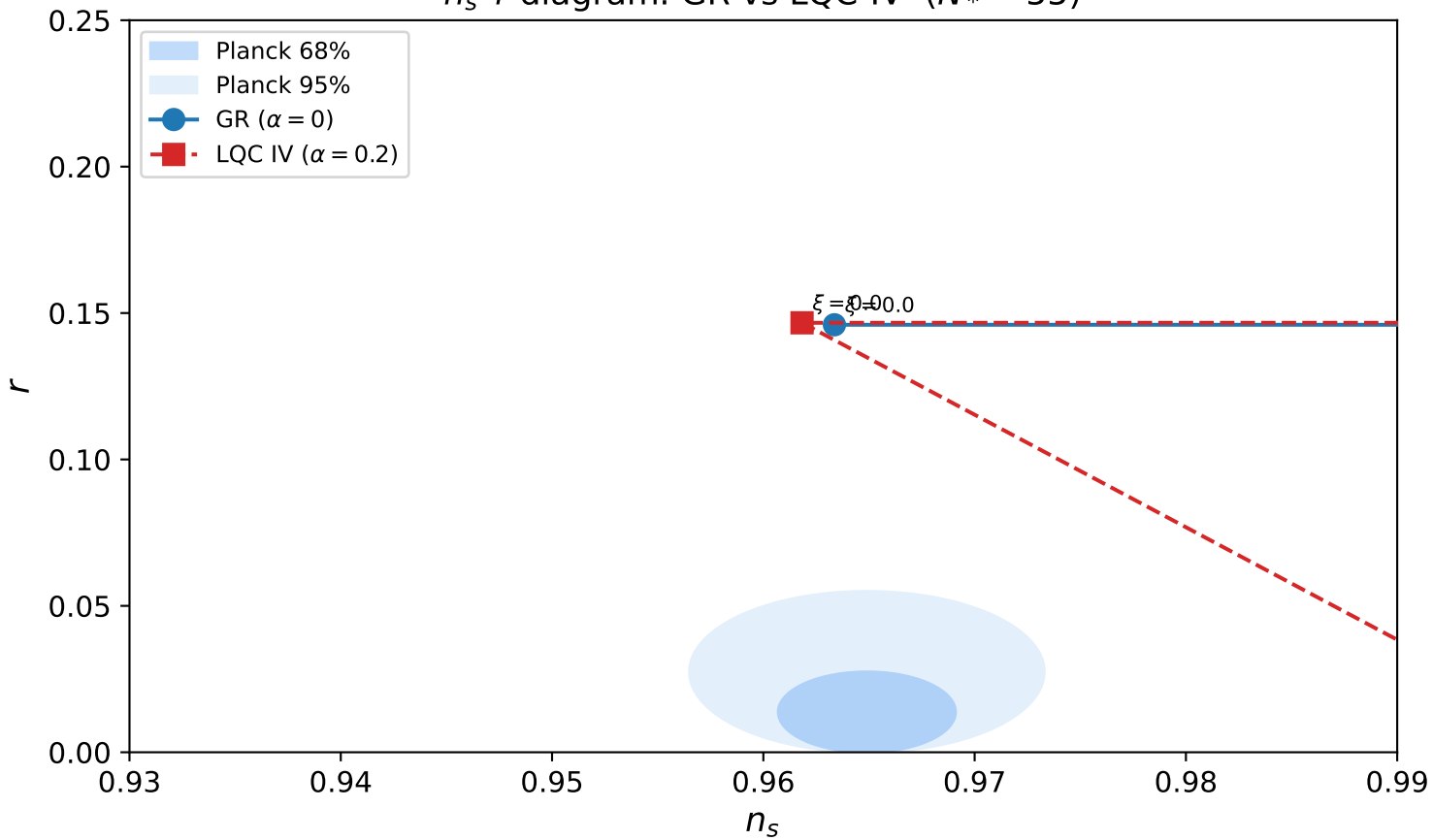
n_s - r diagram: GR vs LQC-IV ( N_* = 55 )
