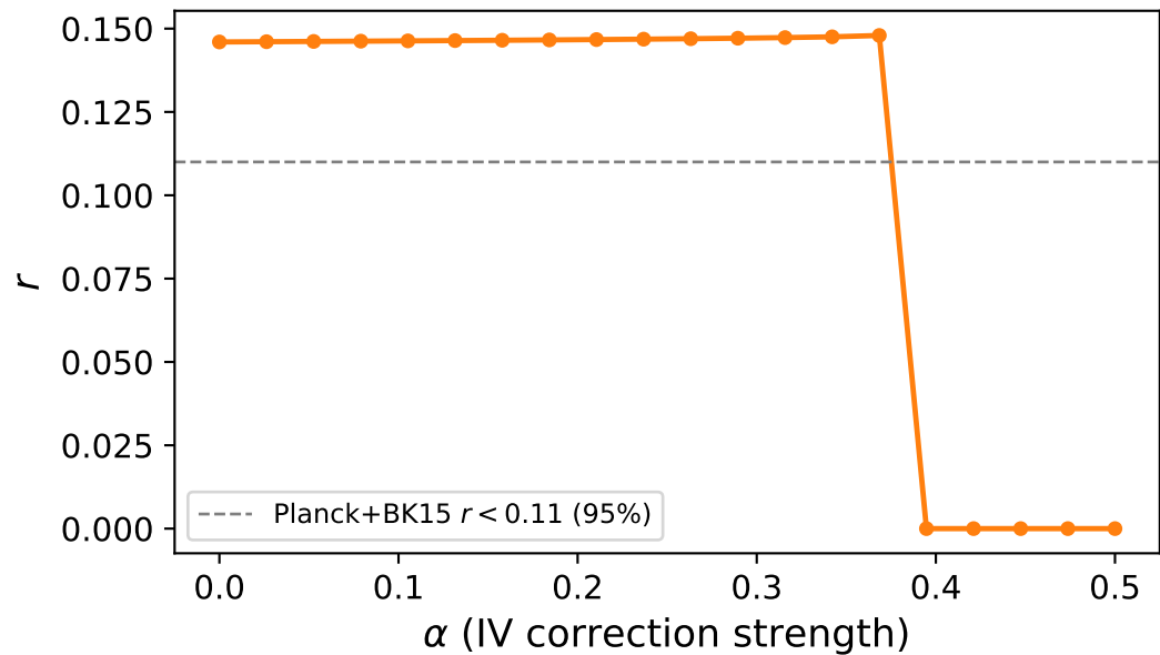
Tensor-to-scalar ratio vs \alpha
