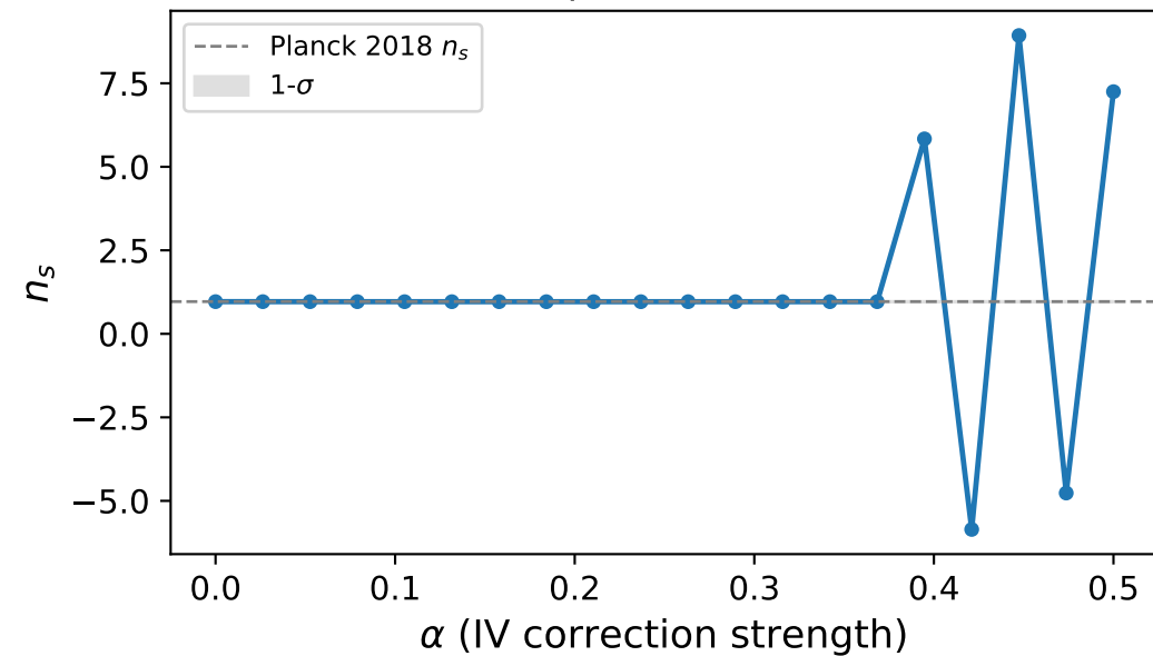
Scalar spectral index vs \alpha
