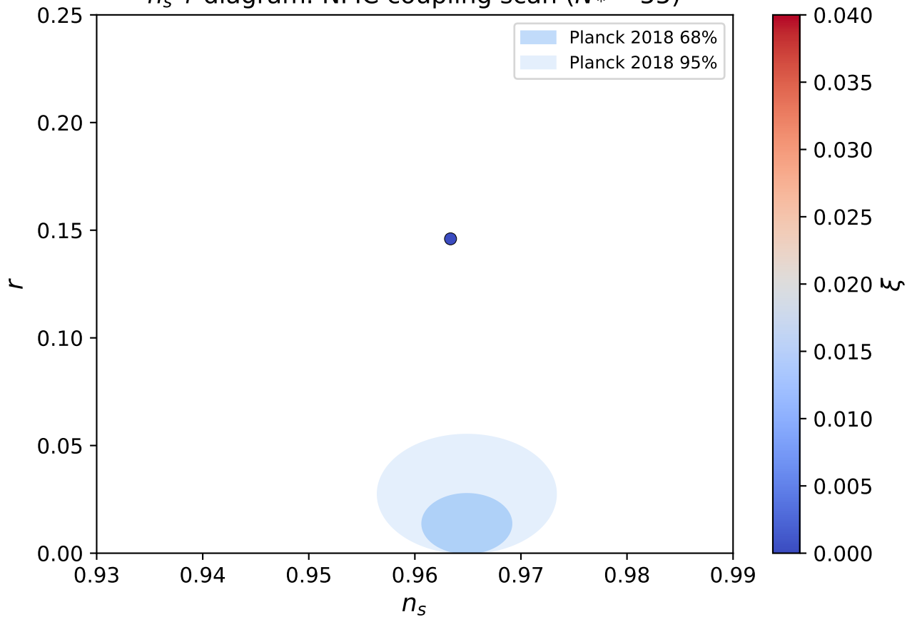
n_s - r diagram: NMC coupling scan ( N_* = 55 )
