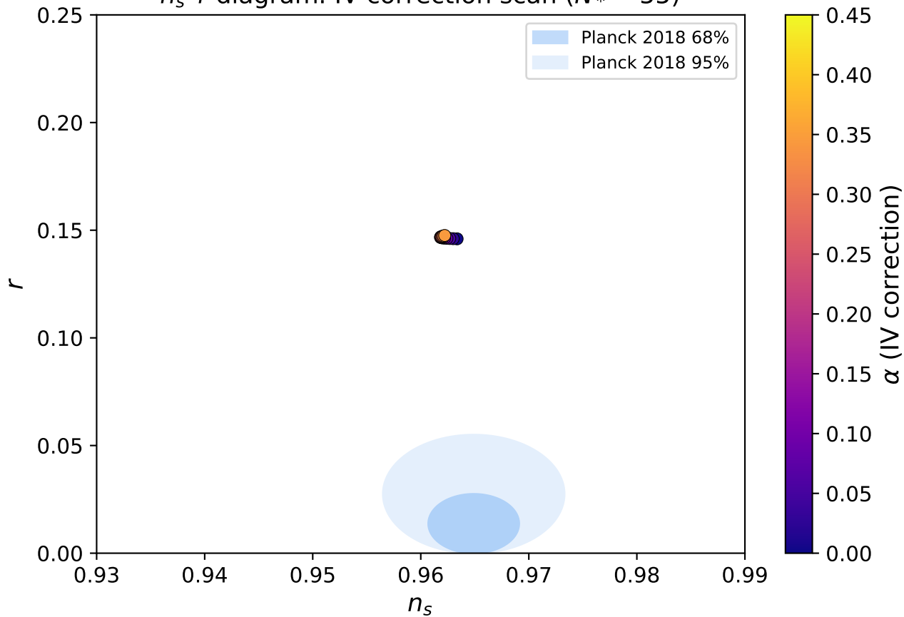
n_s - r diagram: IV correction scan ( N_* = 55 )
