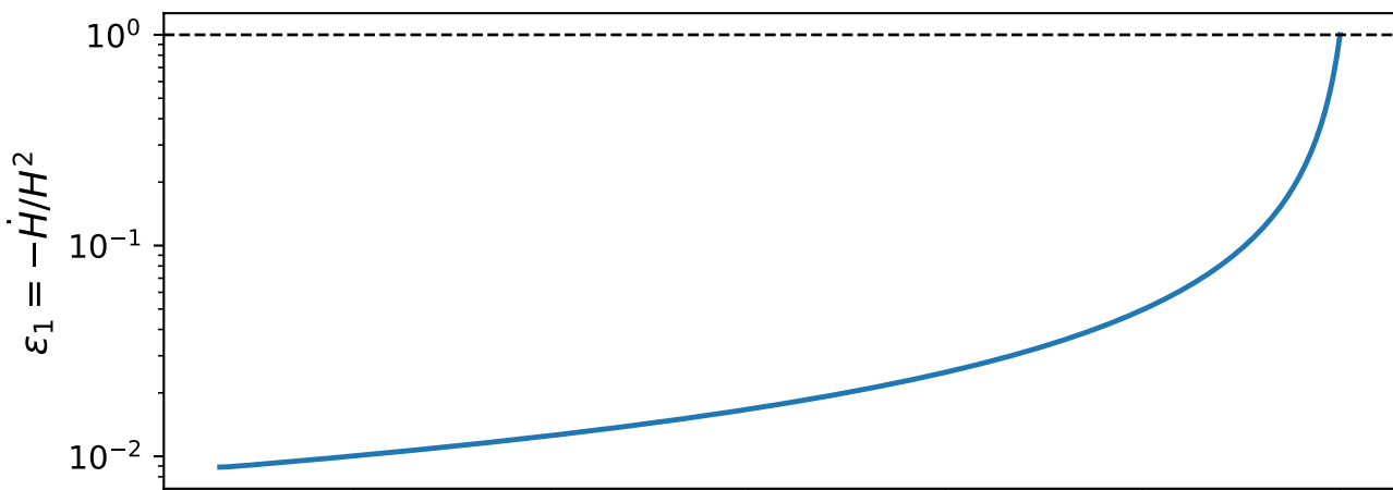
Slow-roll parameters ( \xi = 0.0 , \alpha = 0.0 )
