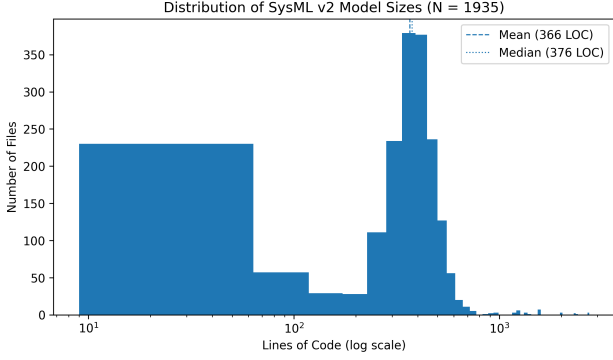
Figure 3. Distribution of SysML v2 model sizes measured in lines of code (LOC), shown on a logarithmic x-axis (N=1935). Dashed and dotted lines indicate the mean (366 LOC) and median (376 LOC), respectively.
