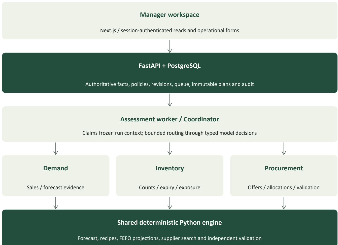
Figure 1. Authoritative data flow. The frontend never receives an Agent token. Specialist outputs return through Backend validation before a new plan is published. External purchase placement remains outside this system. [3]
