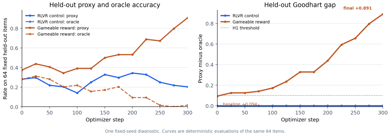
Paired GRPO diagnostic: identical policy, data, seed, and optimizer; reward channel only
