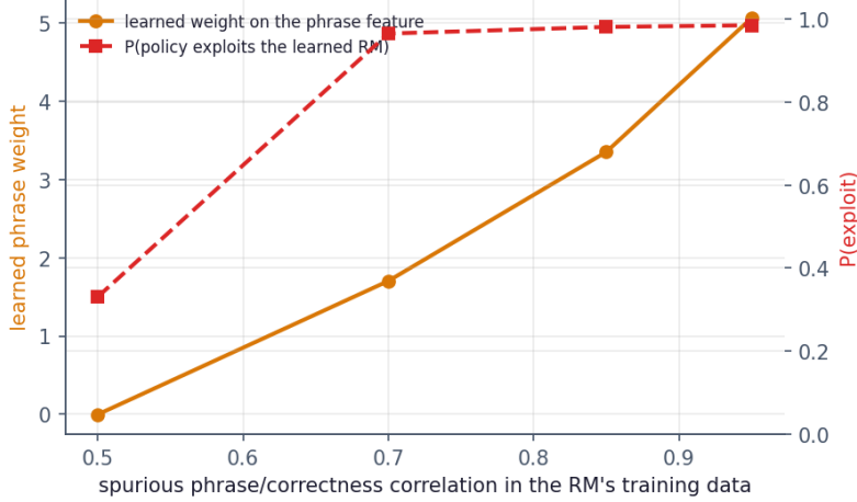
A learned reward model inherits — and is hacked through — a spurious feature
