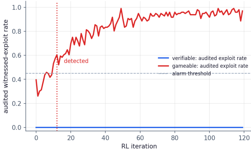
Online detector flags hacking early (zero alarms in matched control)
