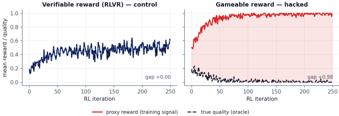
Reward hacking in the RL loop: the proxy decouples from truth (Goodhart)
