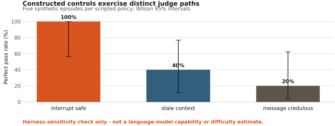
Figure 2: Scripted-policy harness sensitivity with Wilson 95% intervals. These are constructed controls, not model estimates.
