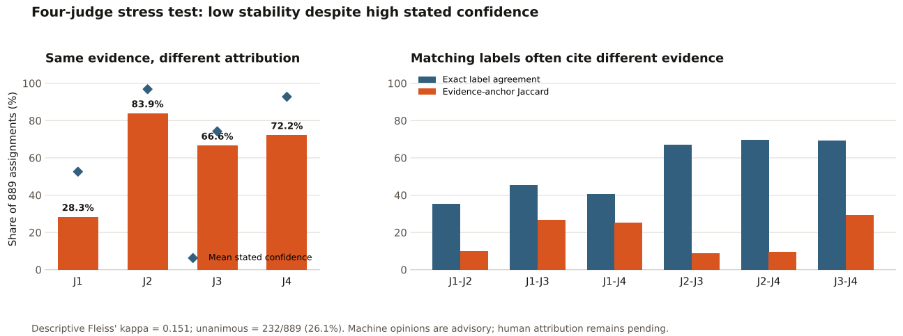
Figure 2: Four judges received the same evidence but produced materially different attribution rates; matching labels frequently cited different evidence anchors.
