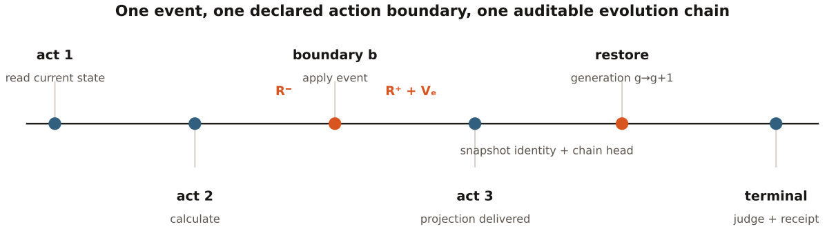
Figure 1: One witnessed episode binds logical boundaries, before/after roots, the actor-visible projection, restore generation, and terminal judgment.
