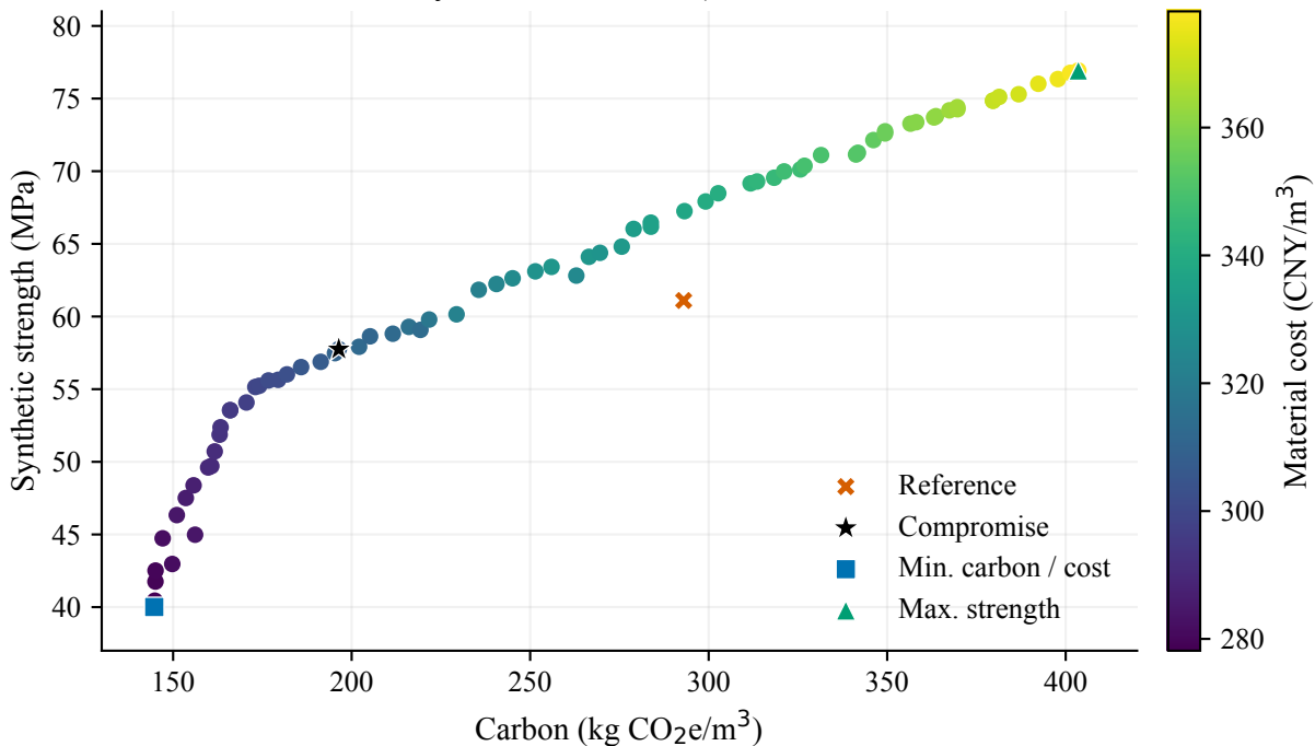
Synthetic Pareto set | seed 42
