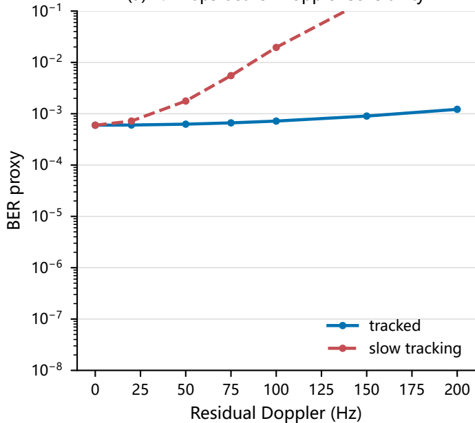
(a) 2.4 kbps bearer Doppler sensitivity
