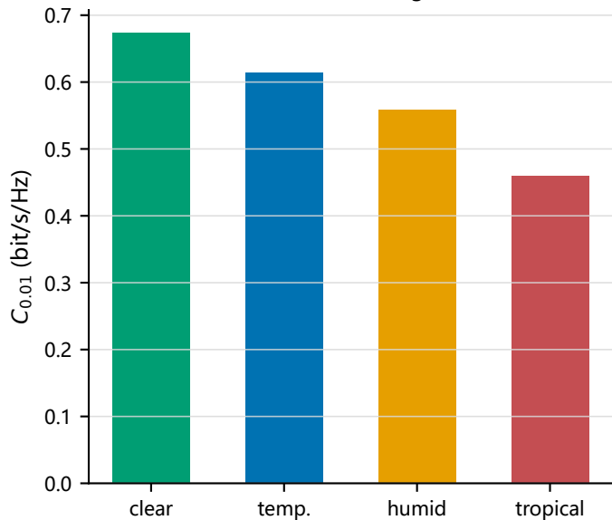
(b) S-band rain-margin shift
