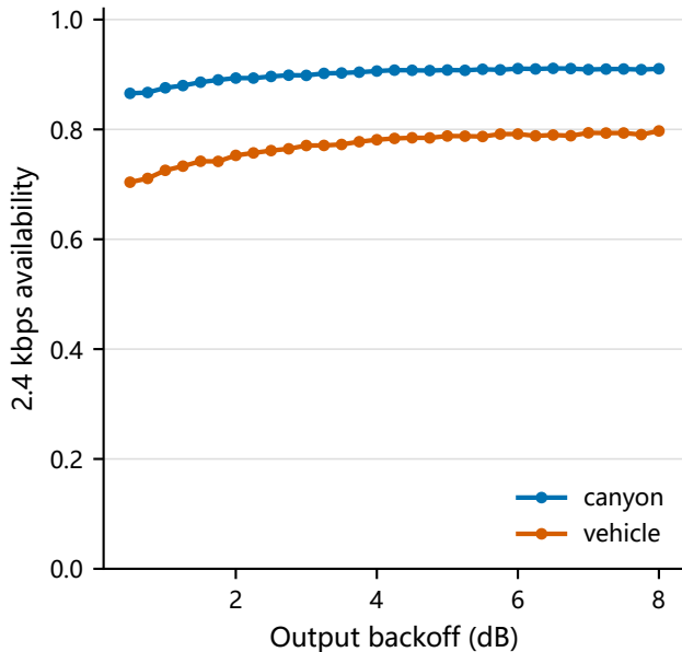
Voice availability under PA loss
