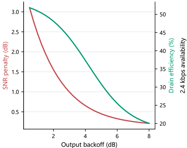
PA compression and ET proxy
