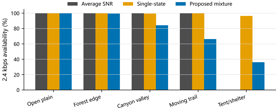
Average-SNR and single-state screening distort low-tail availability
