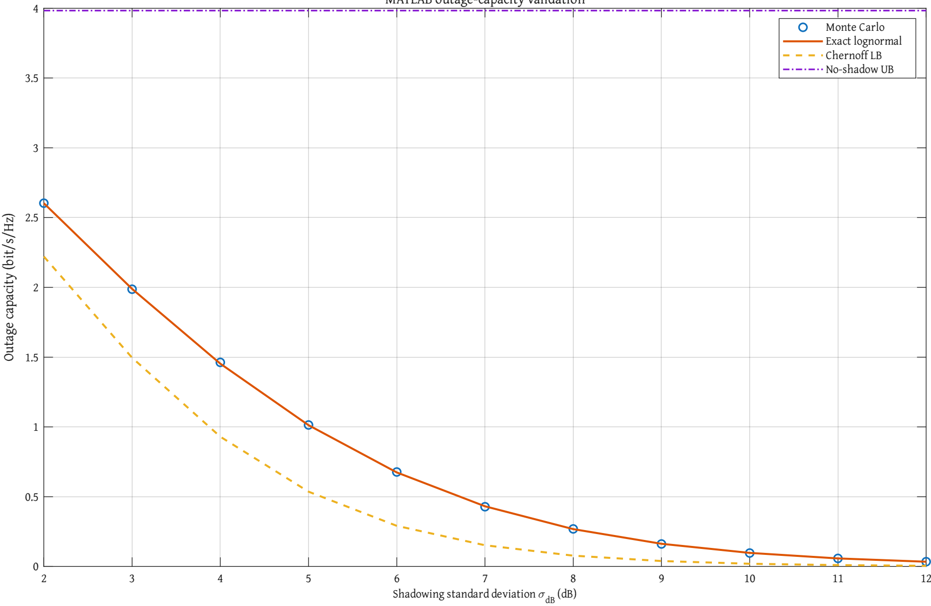
MATLAB outage-capacity validation
