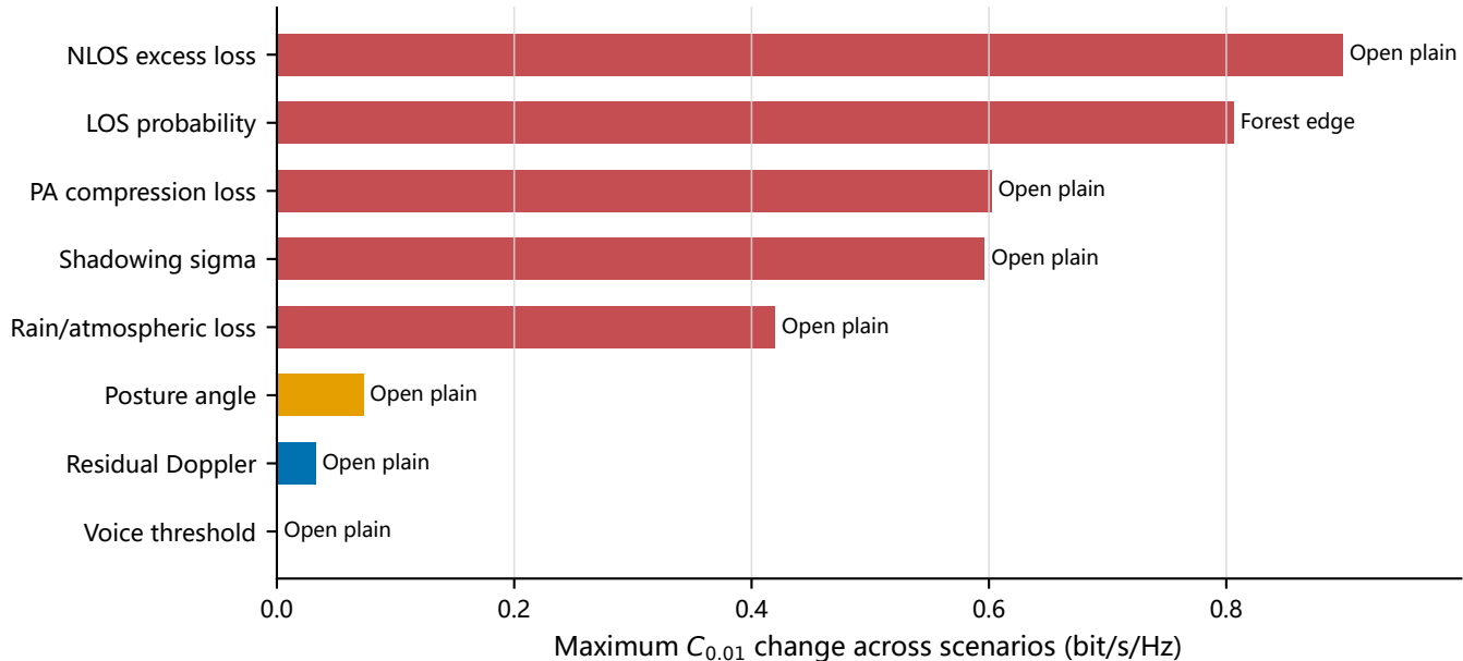
Global C_{0.01} sensitivity ranking
