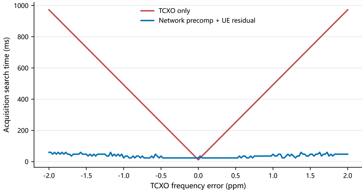
Two-stage frequency compensation proxy
