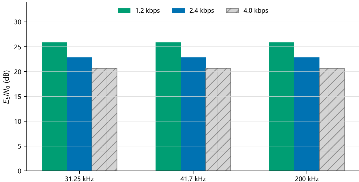
GEO S-band narrowband bearer link budget
