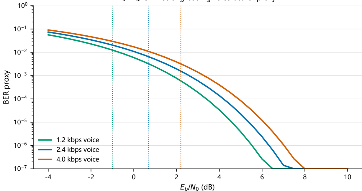
\pi/4 -QPSK + strong-coding voice bearer proxy
