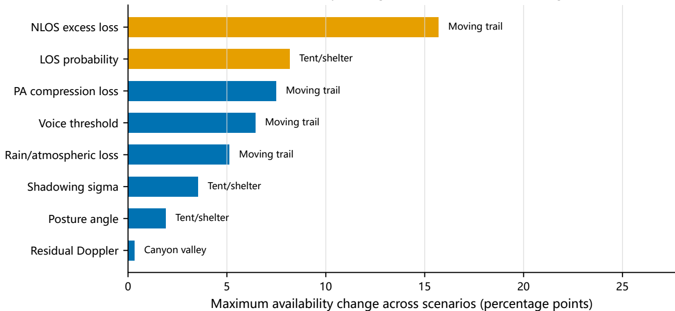
Global sensitivity ranking for 2.4 kbps low-tail screening
