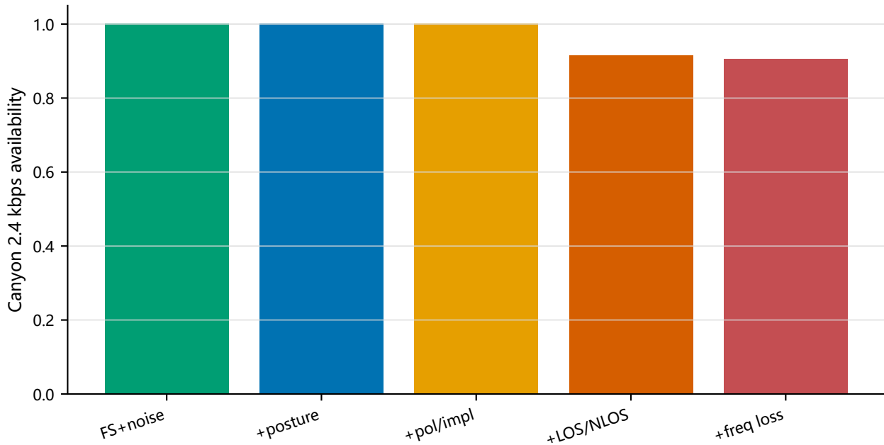
Cumulative impairment ablation
