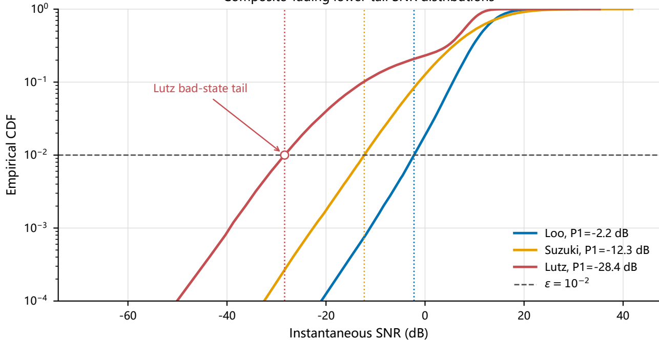
Composite-fading lower-tail SNR distributions
