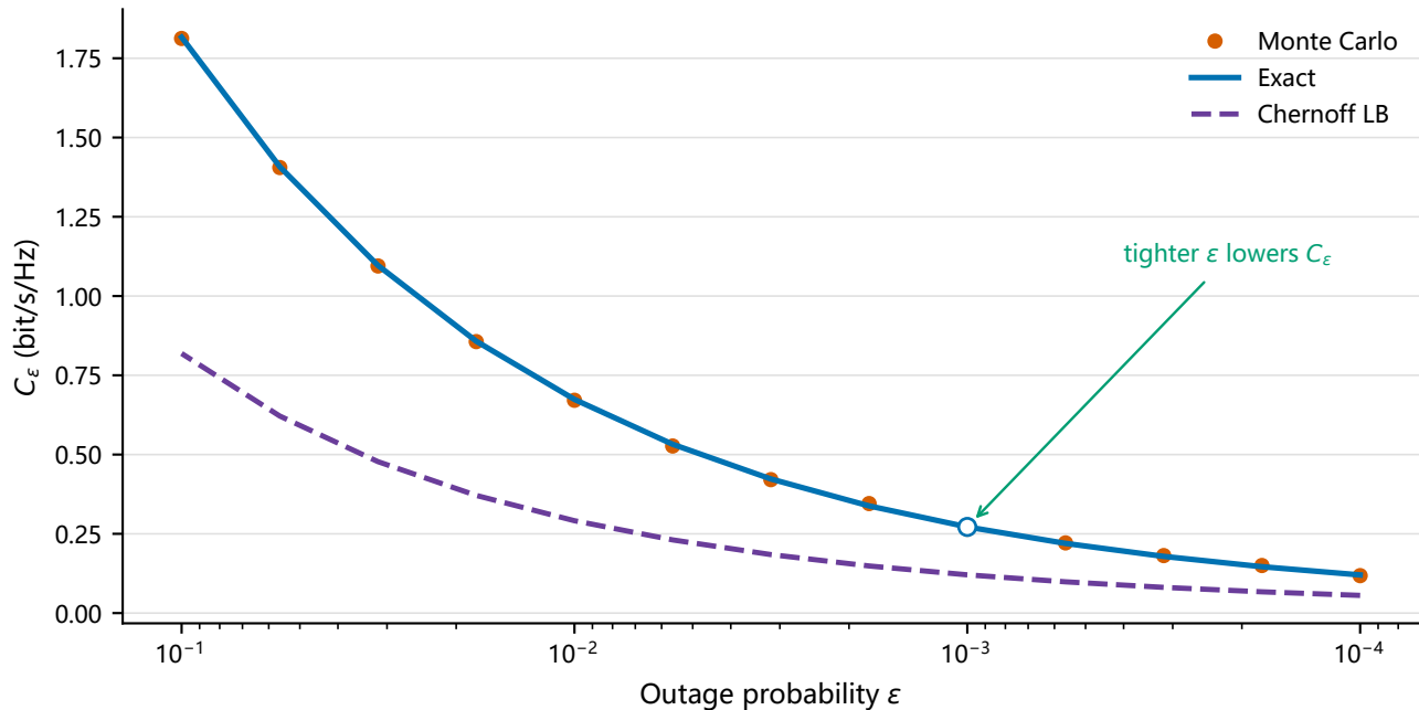
Outage target scaling, \sigma_{dB} = 6 dB
