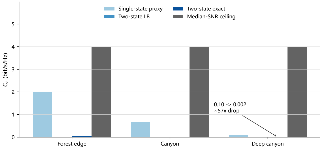
LOS/NLOS mixture penalty, \varepsilon = 10^{-2} , elevation 45^\circ
