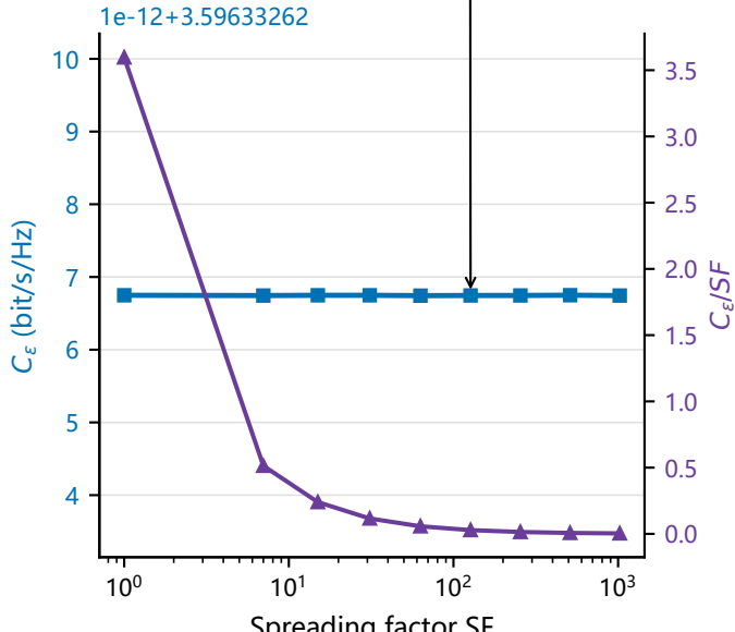
(b) Bandwidth-consistent: no SF leverage
