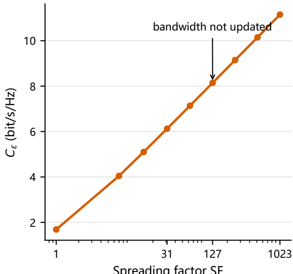
(a) Fixed 5 kHz bandwidth: illusory gain
